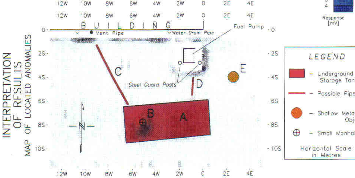
GEONICS EM61 SURVEY OF A SITE WITH AN UNDERGROUND STORAGE TANK
